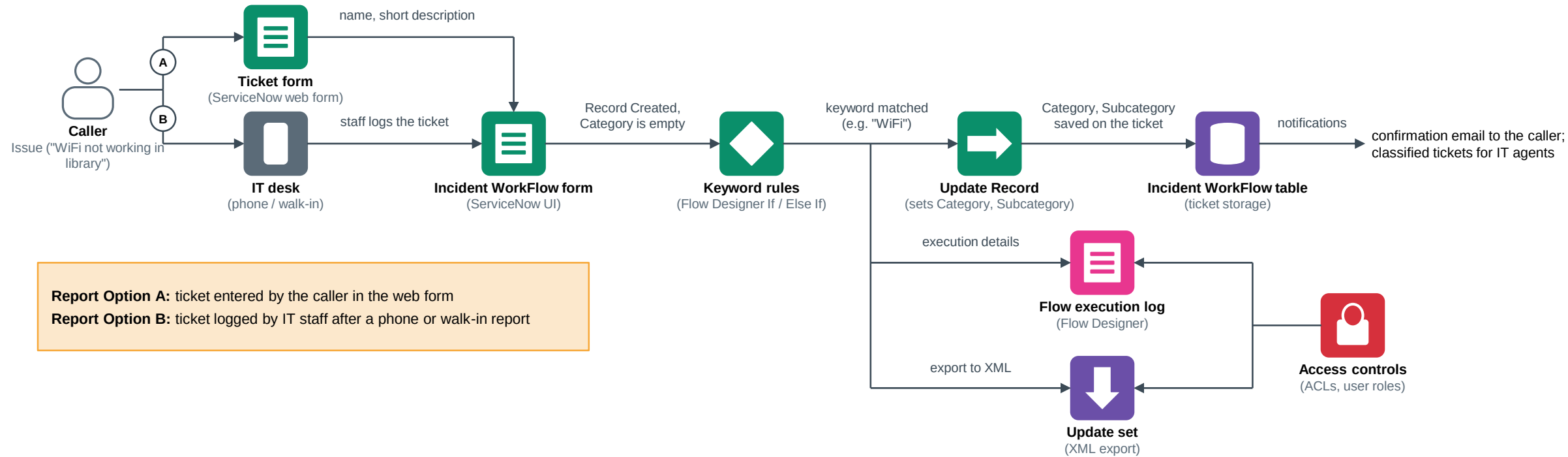
Figure 1: Architecture and data flow of the Auto Ticket Classification solution
